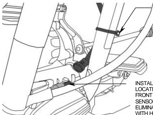
FIGURE 5 (‘07 - ‘10 SOFTAIL)
