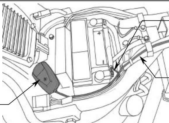
FIGURE 4 (‘07 - ‘10 SOFTAIL)
